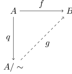
Figure 1.10: A commutative diagram illustrating the quotient factorization theorem for sets. A commutative diagram is a diagram of objects and functions in which any two paths with the same start and end points yield the same output for each input.
